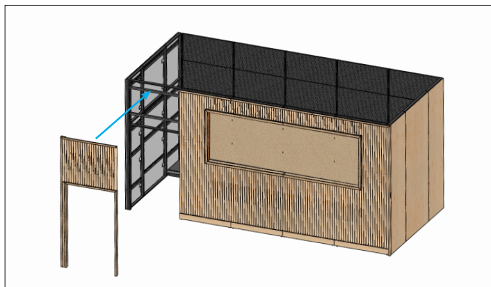
Step 14: Hang Left Panel Assembly over the door frame area. Ensure all z hangers are interlocked.
