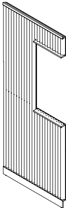
48IN LEFT PANEL ASSEMBLY (QTY 1) SUB56769
