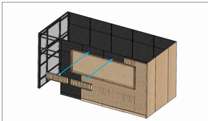
Step 12: Hang Upper Panel Assemblies (x2) above TV Frame .
