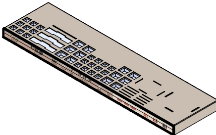
BDB MIDDLE SHELF (QTY 1)
