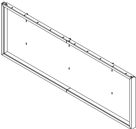
TV FRAME ASSEMBLY (QTY 1) SUB56770
