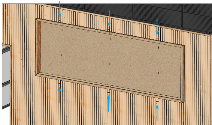
Step 15: Behind the front edge of the TV frame, add Connection Plates (x6) over seams to secure.
