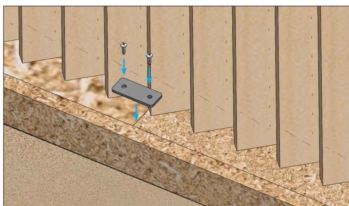
Step 16: Use Screw, #6 x 1/2 Philips to secure each plate.
