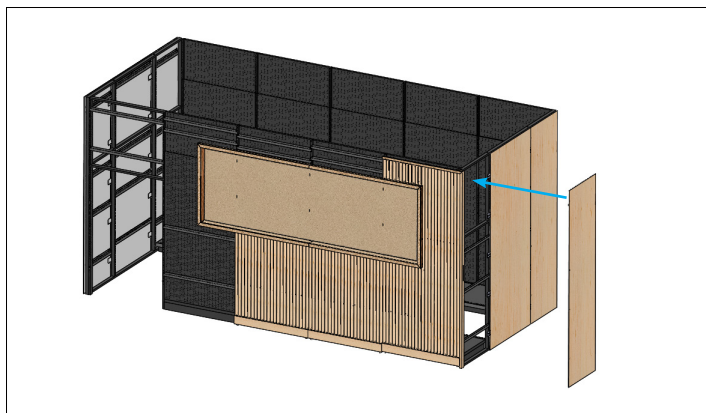
Step 11: Hang last Outside Panel on right side of gondola.
