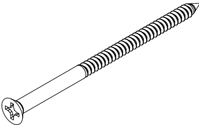
SCREW, #8 X 3" PHILIPS (QTY 2) HWD13718
