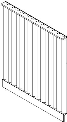
LOWER PANEL ASSEMBLY 1 (QTY 1) SUB56756
