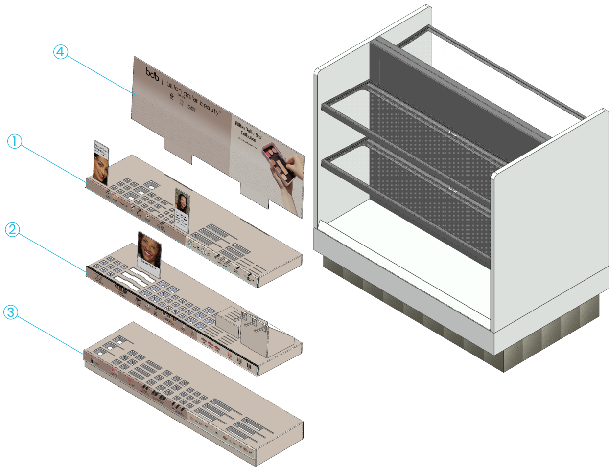
Exploded Isometric View
