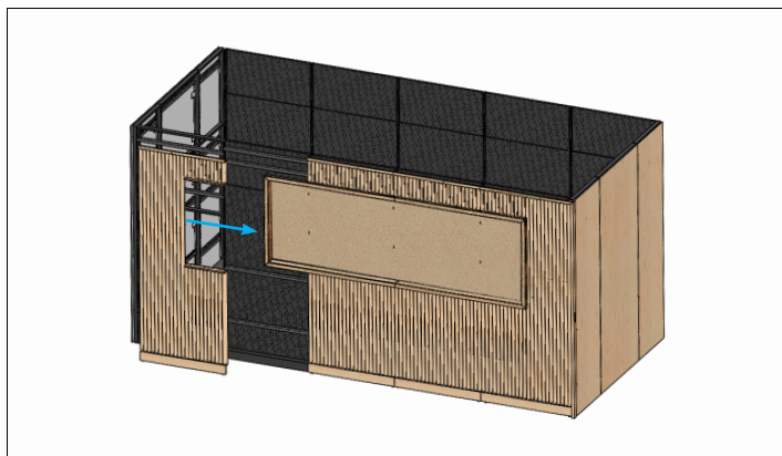
Step 13: Slide on 48in Left Panel Assembly from left side.
